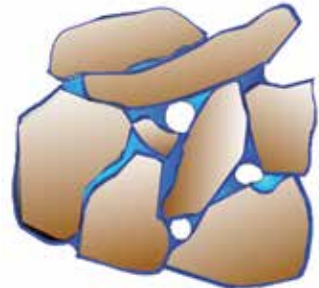
Figure 5.3. A moist sand with pores between grains that contain water and air. The larger pores have partially drained and allowed air entry, while the narrower ones are still filled with water.
